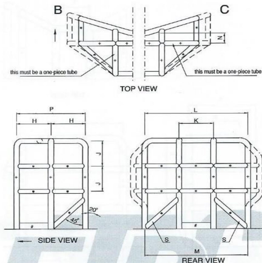
Illustration 14-2: driver roll-over protection B/C
