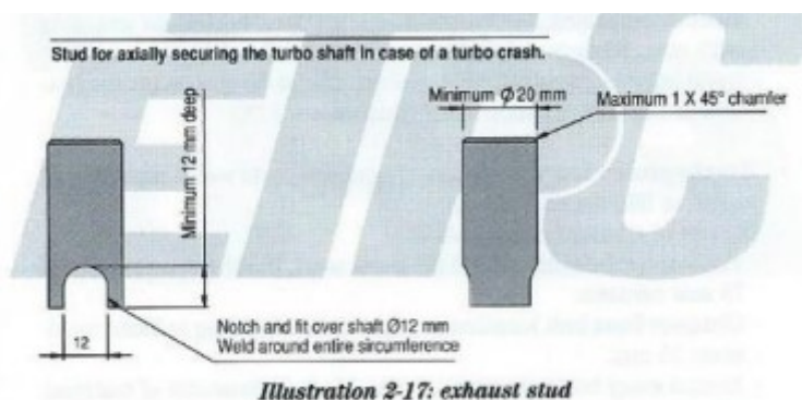
Illustration 2-17: exhaust stud
