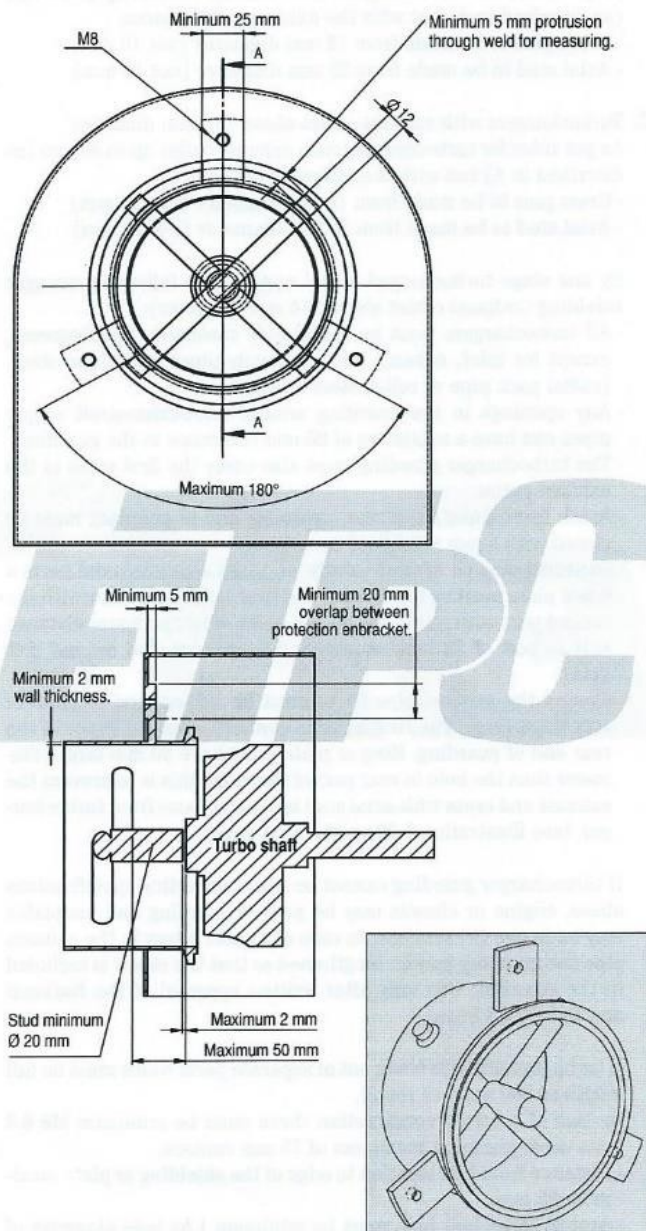
Illustration 2-18: additional connections exhaust pipe
