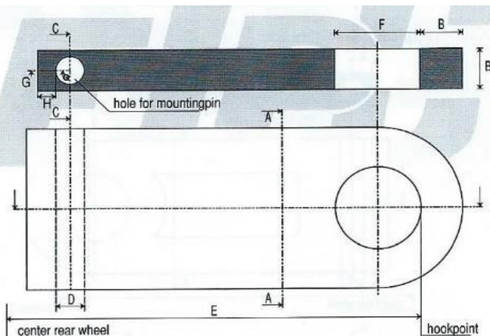
Illustration 2-3: dimensions drawbar Modified <950 kg
