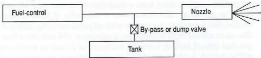
Illustration 2-12: overspeed shutdown on turbine-engines
