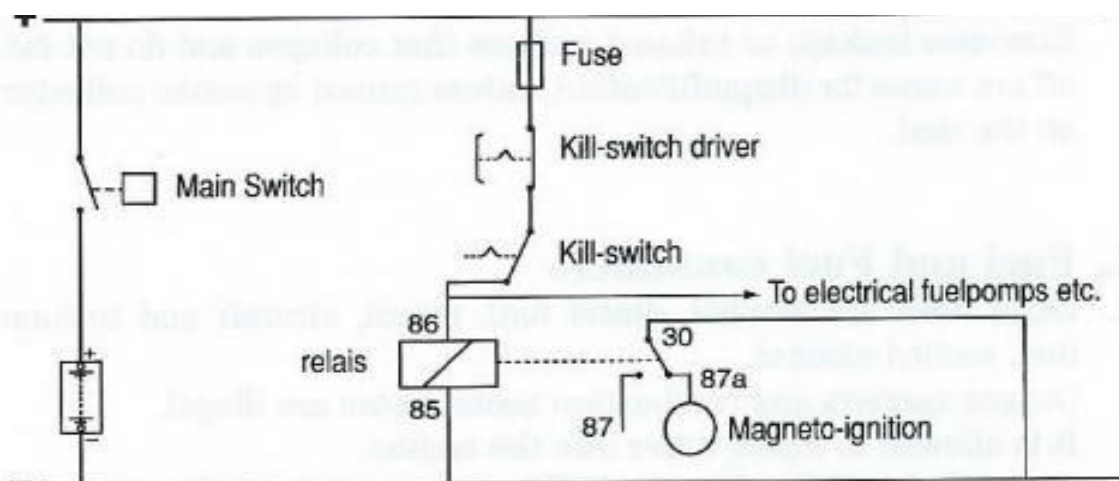
Illustration 2-33: fail safe kill-switch
