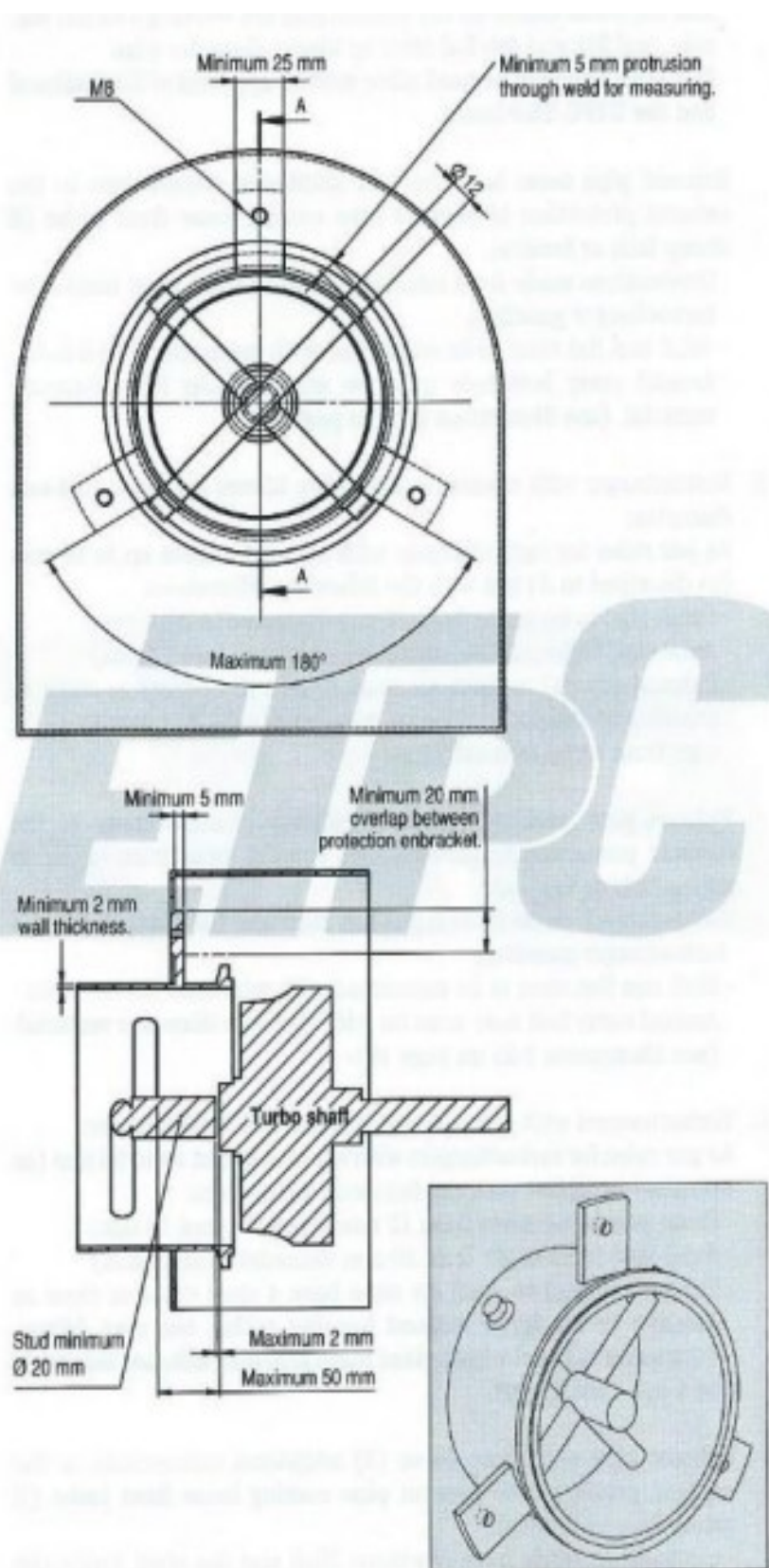
Illustration 2-27: additional connections exhaust pipe
