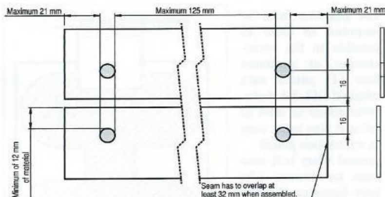
Illustration 2-25: material-overlap in bolted shielding
