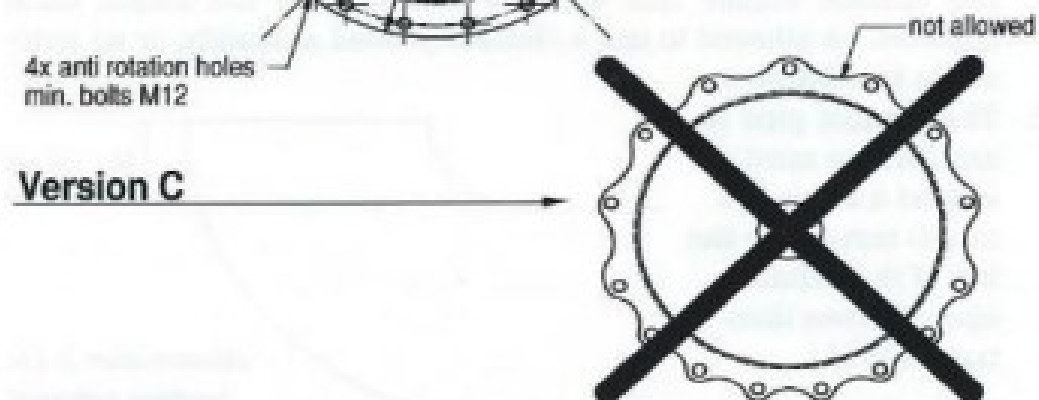
Illustration 2-10: aluminum bellhousing
